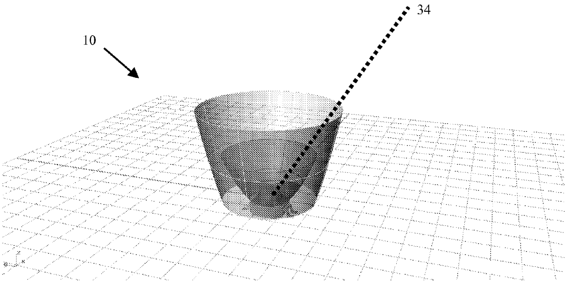
Figure 3: Multi-stage reflector in fully retracted position
