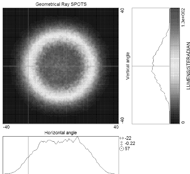
Figure 13 – “FAR” or “WIDE” POSITION: 1.3 CD/LM MAXIMUM
