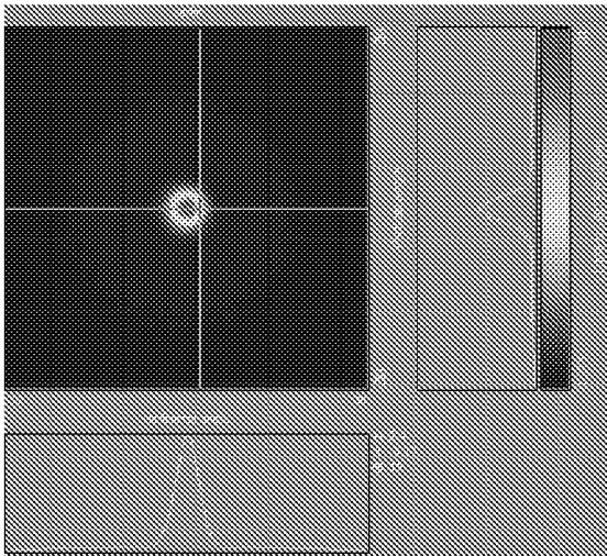
Figure 32: narrow beam - intensity vs. angle
