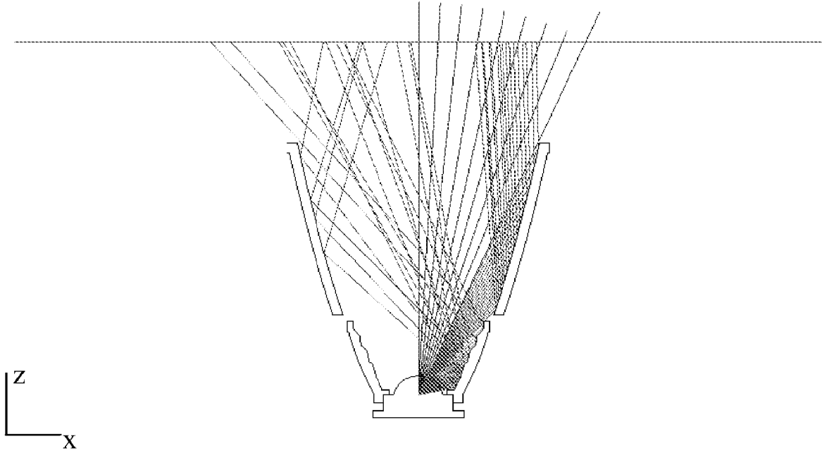
Figure 29: outer reflector (and inner) ray path details
