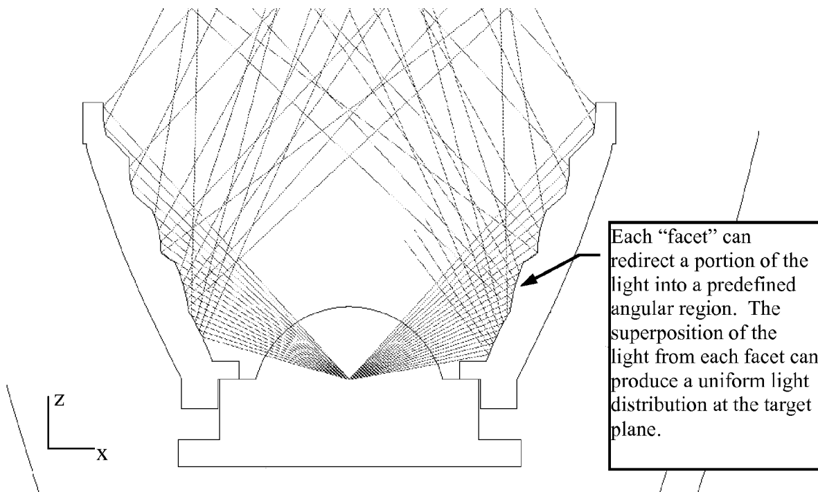
Figure 28: inner reflector ray path close-up
