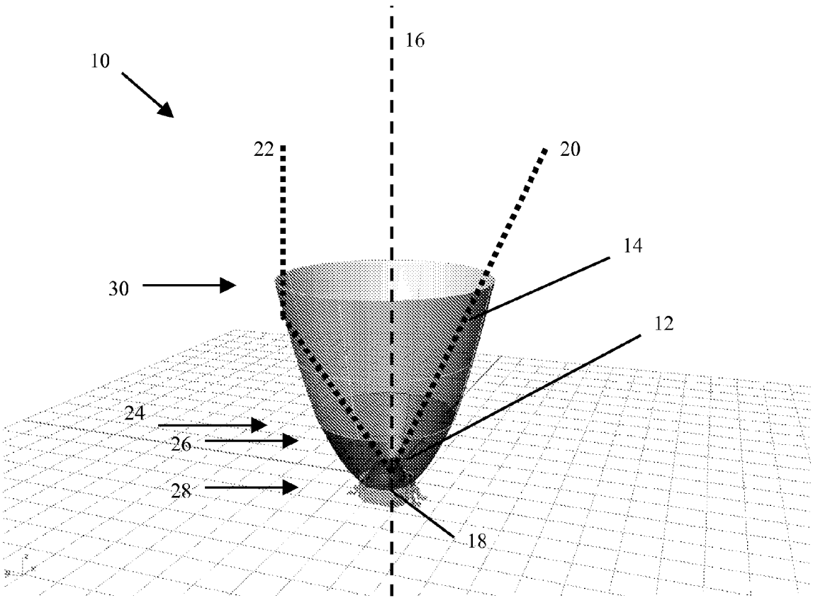
Figure 1: Multi-stage reflector in fully extended position
