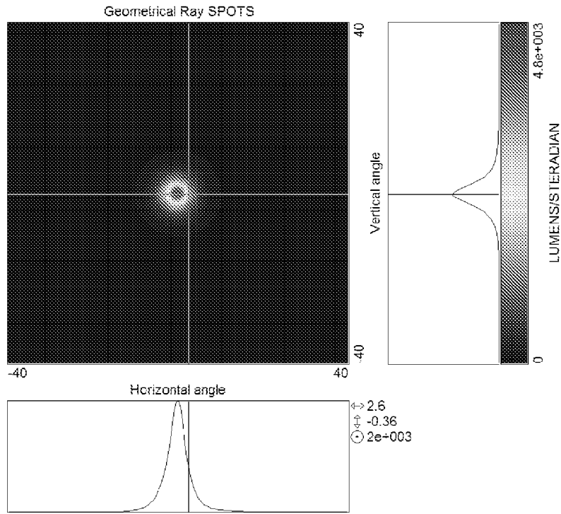
Figure 12 – “CLOSE” or “NARROW” POSITION: 48 CD/LM MAXIMUM
